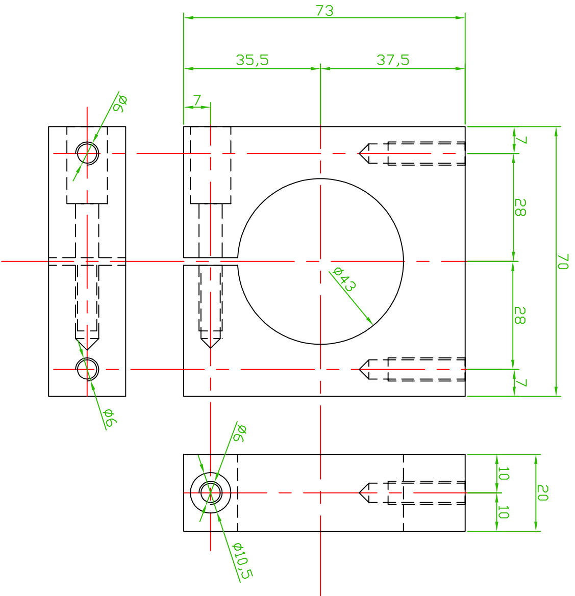
Support Broche
